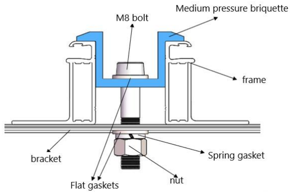
Figure 17 Installation schematic diagram of mid clamp
