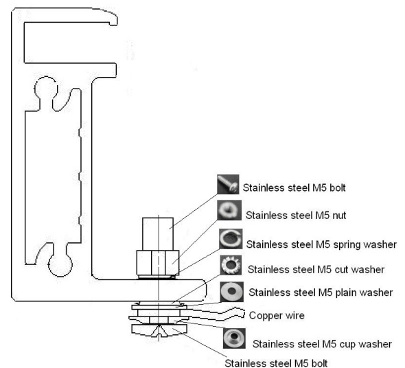
Fig. 19 Grounding the aluminum frame with copper wire
