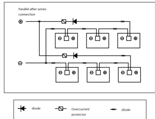
Fig. 18 Schematic diagram of electrical connection
