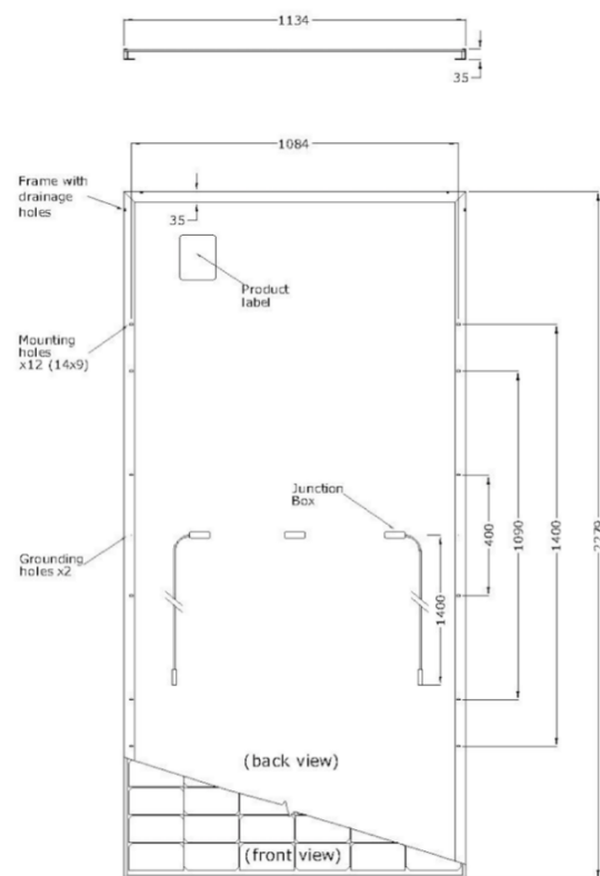
Fig. 6: Mechanical drawing of the FU XXX M / MV SILK® PLUS (144 half-cut cells) module showing the mounting holes, the drainage holes.
