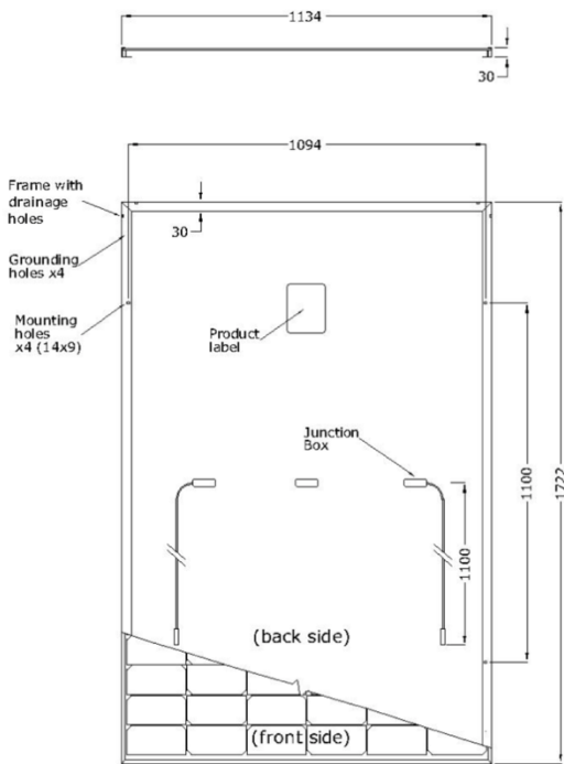
Fig. 5: Mechanical drawing of the FU XXX M / MV SILK® PLUS (108 half-cut cells) module showing the mounting holes.
