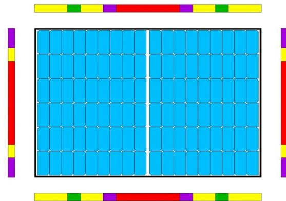
Fig. 4: Positions for clamping and fixing SILK® PLUS module series
