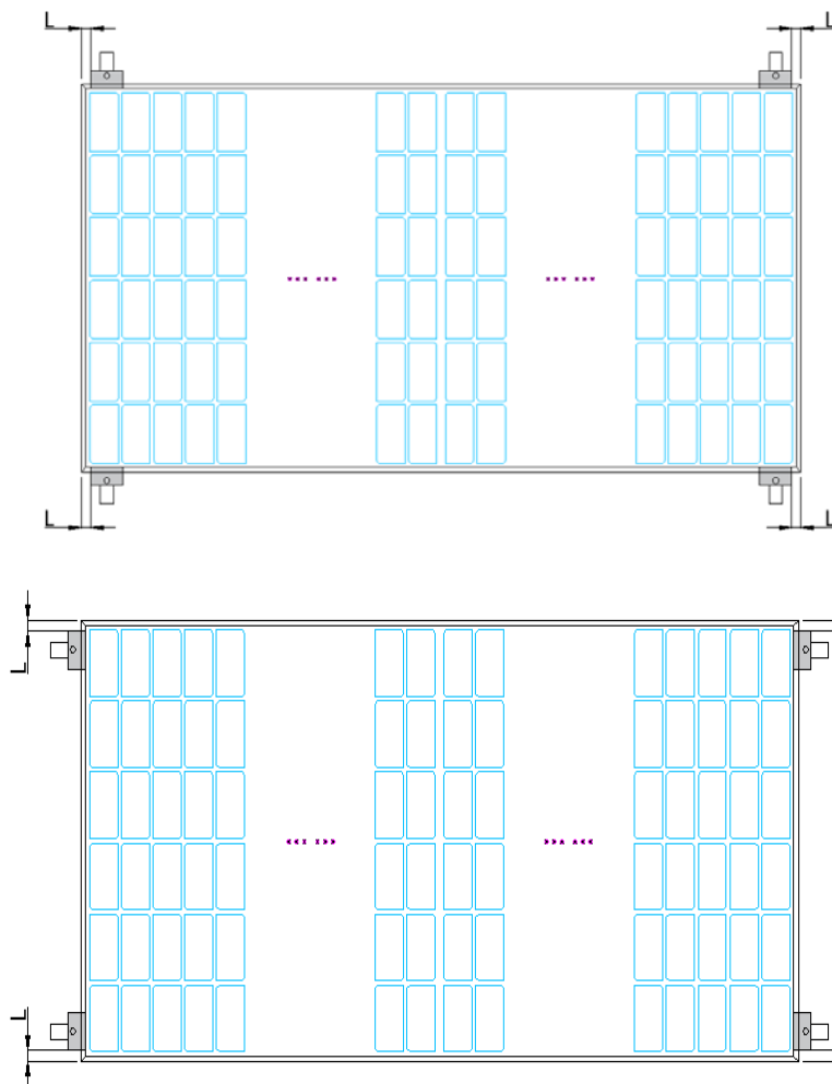
Figure 11-1: clamps fixed method in long side
